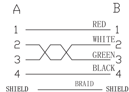
PIN ASSIGNMENT
