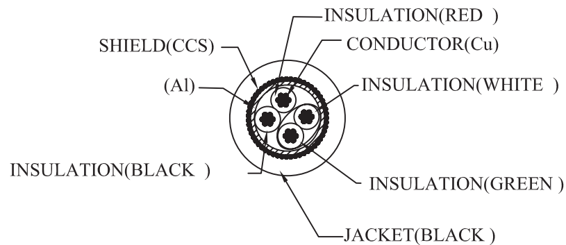
Cable Sketch Map
